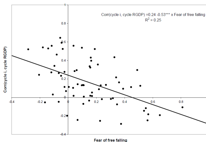
Figure 15. Country correlations between the cyclical components of short-term interest rate and real GDP vs. fear of free falling. 1960-2009
