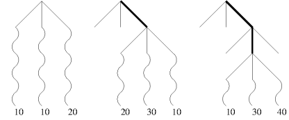
Fig. 1. At each step of the principal payout shown here with a bold line, a NMCS of level n performs a NMCS of level n - 1 (shown with wavy lines) for each available move and selects the best one. At level 0, a simple pseudo-random payout is used.
