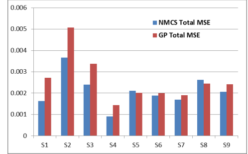
Fig. 3. Performance of the generated NMC and GP volatility models according to "MSE total"
